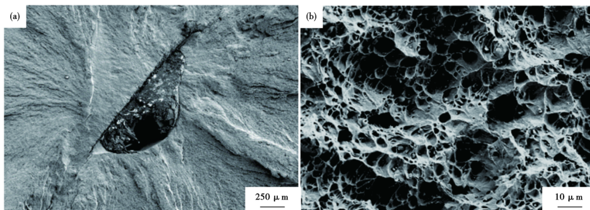
图 9 应力水平为 380 MPa 时 FH420 钢气保焊焊接接头断口形貌: (a) 裂纹源区, (b) 断裂区 Fig. 9 When the stress level is 380 MPa, the fracture morphology of FH420 steel gas shielded welding joint : (a) crack source area, (b) fracture zone
